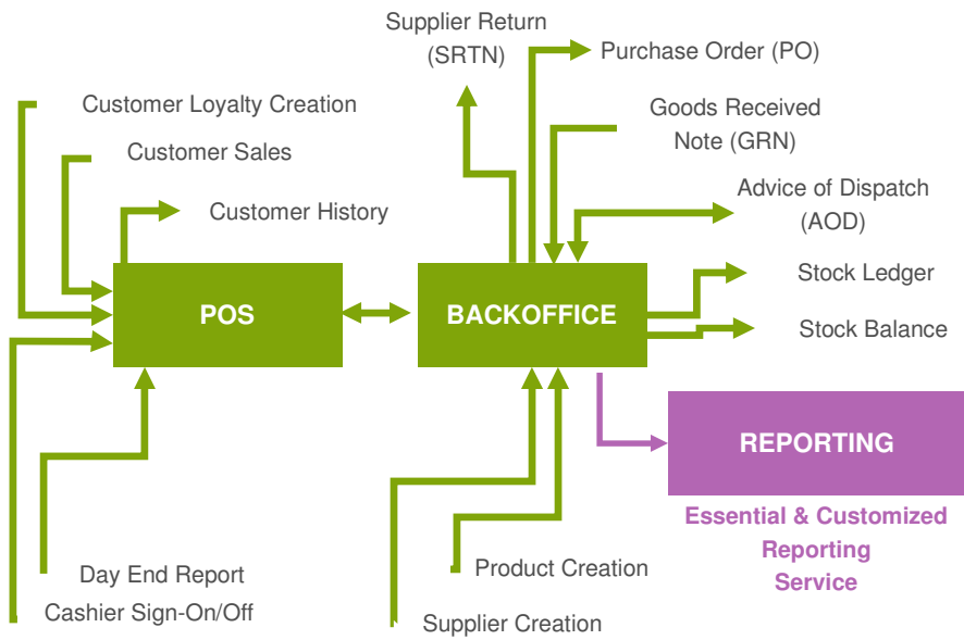
ELEGRA APPs — POS MIS SYSTEM CORE STRUCTURE
